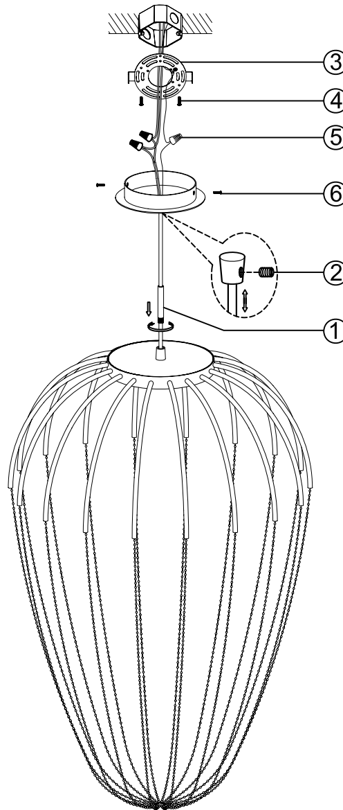
Wire connection
